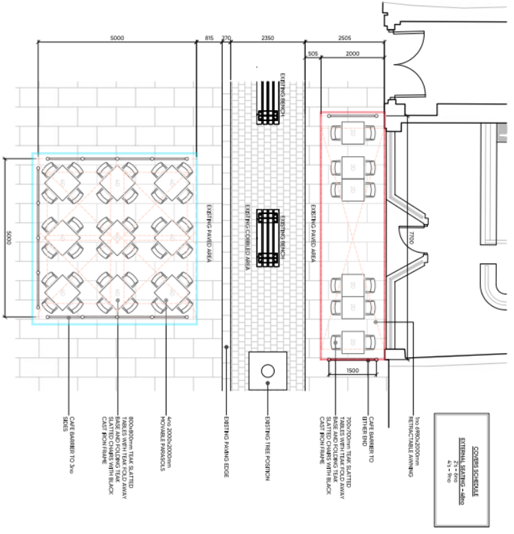
EXTERNAL LAYOUT / PAVEMENT LICENSE PLAN Scale 1:50 = A1 / 1:500 = A2
