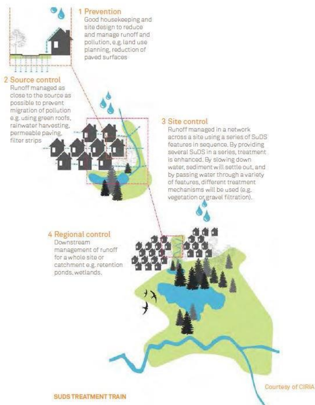
Figure 7-2 SuDS management train
