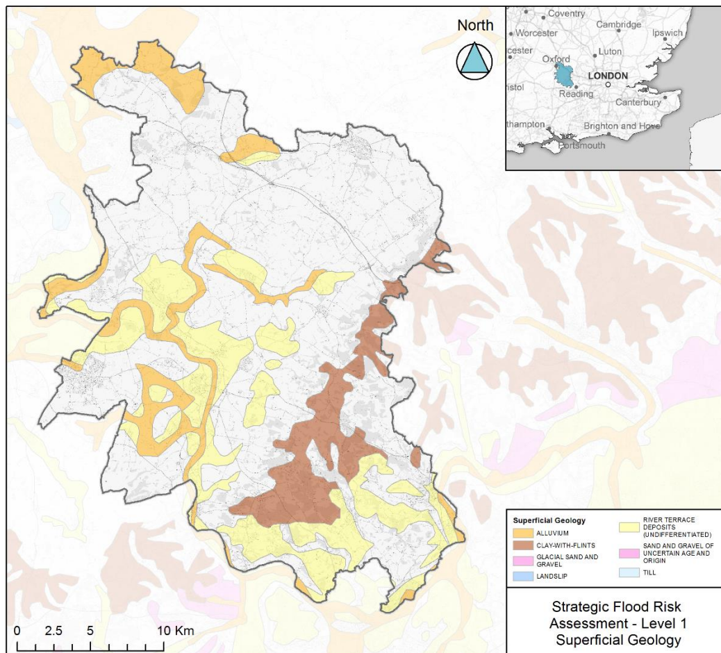
Figure 5-2 Superficial geology in SODC area
