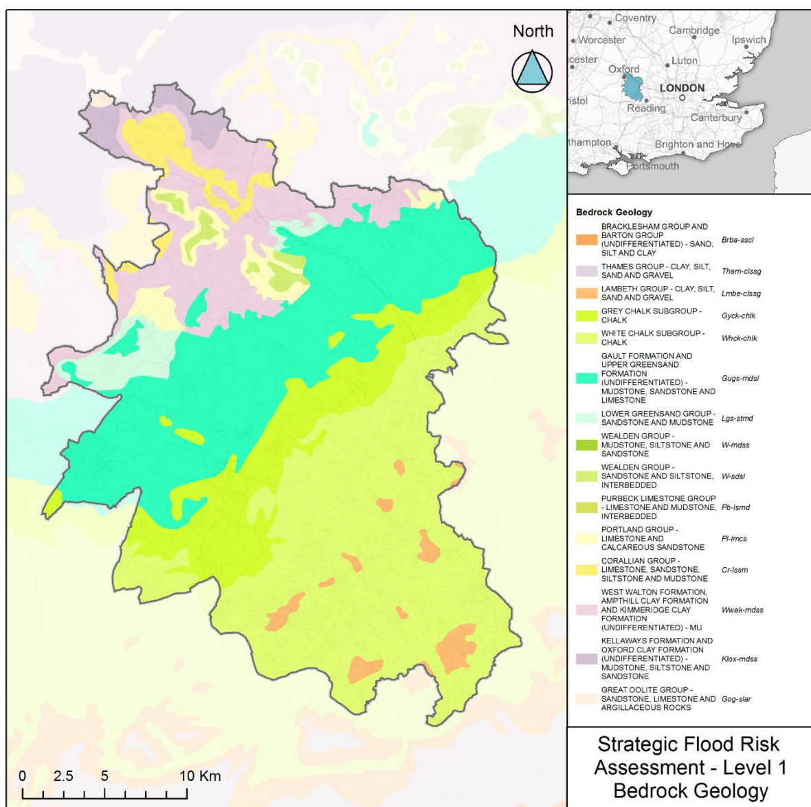
Figure 5-3 Bedrock geology of the SODC area
