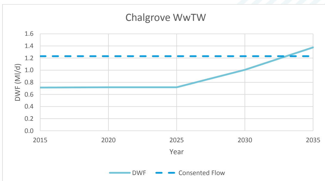
Figure 5-4: Flow permit assessment for Chalgrove WwTW
