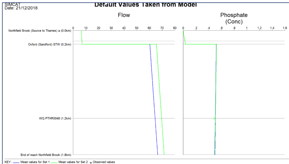
Figure A-7: Plot of deterioration, flow and phosphate
