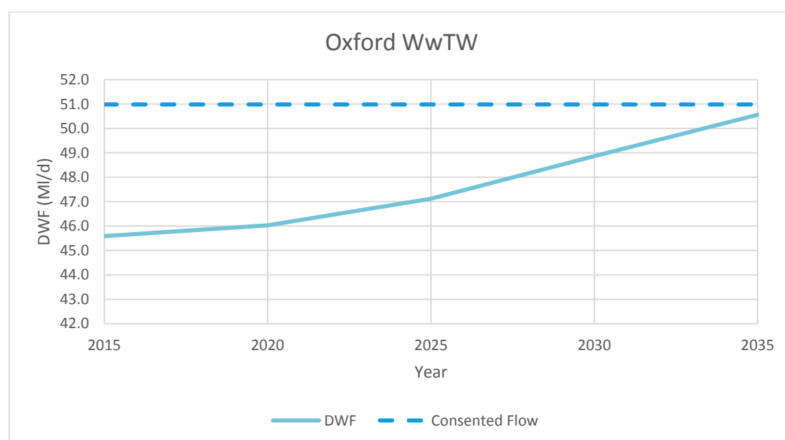
Figure 5-2: Flow permit assessment for Oxford WwTW
