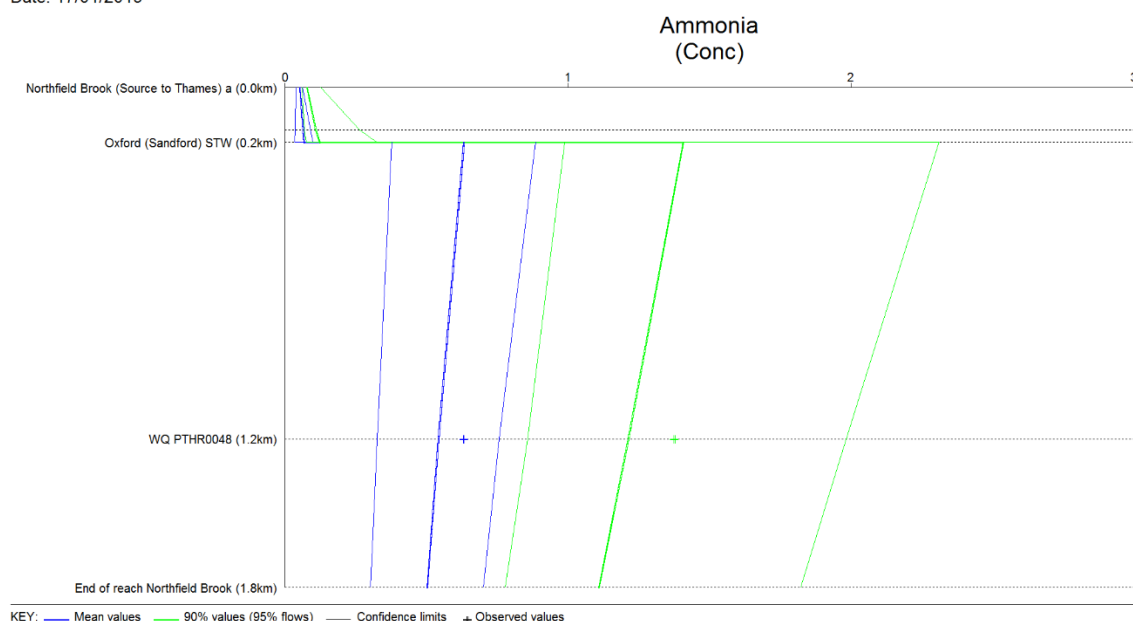
Figure A-4: Northfield Brook baseline ammonia
