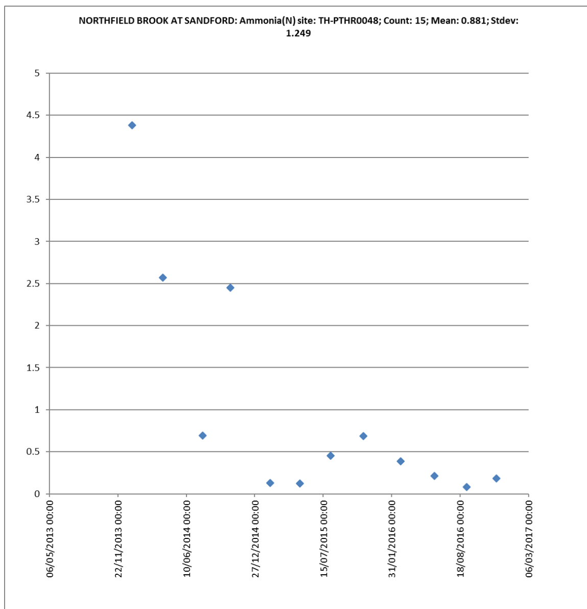
Figure A-3: Northfield Brook at Sandford observed Ammonia samples
