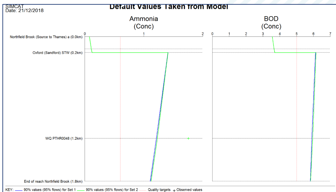
Figure A-6: Plot of deterioration, ammonia and BOD
